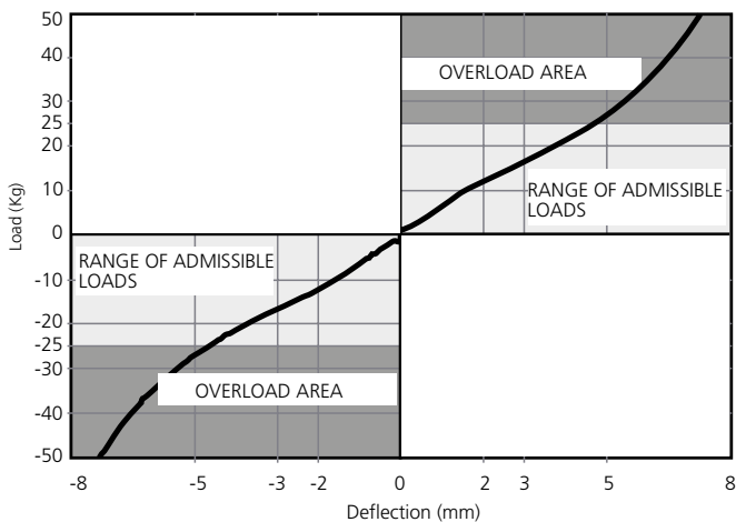
LOAD DEFLECTION GRAPH EP Akustik + Sylomer 25
