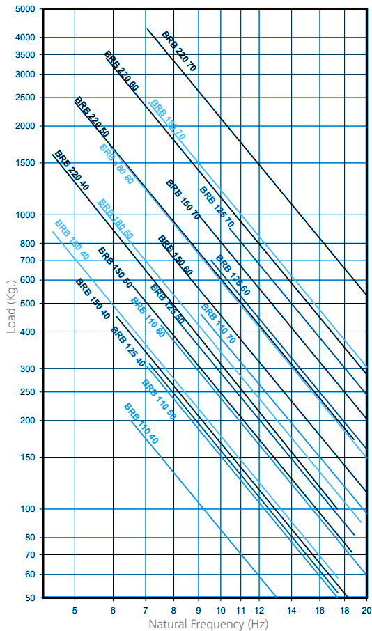
NATURAL FREQUENCY AMC MECANOCAUCHO® BRB 110-220 TYPE
